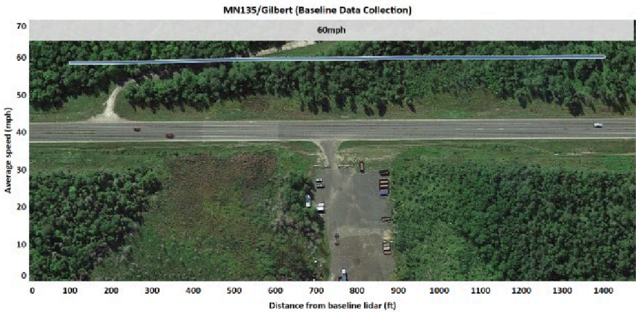
Figure 17 Average Speed Profile as Vehicles Transit through 60 mph Speed Zone on MN135/Gilbert Corridor
