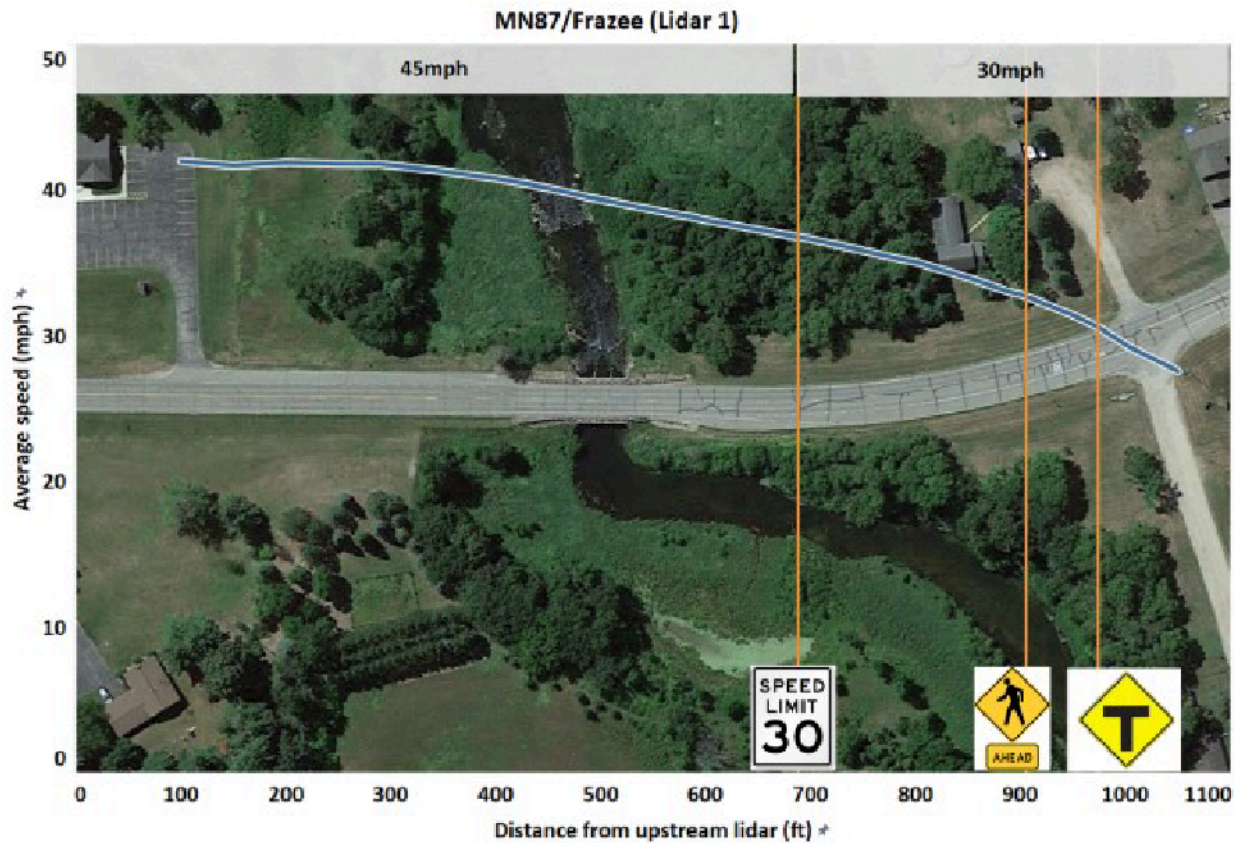
Figure 32 Average Speed Profile as Vehicles Transit from 45-30 mph on MN87/Frazee Corridor
