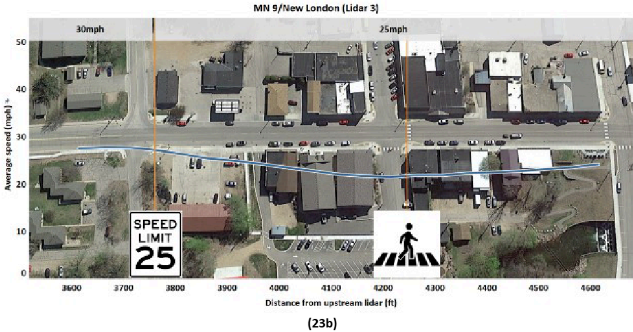
Figure 23 Average Speed Profile as Vehicles Transit from 45-30-25 mph on MN9/New London Corridor
