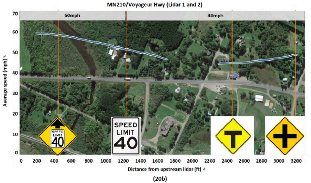
Figure 20 Average Speed Profile as Vehicles Transit from 60-40 mph on MN210/Voyageur Hwy Corridor
