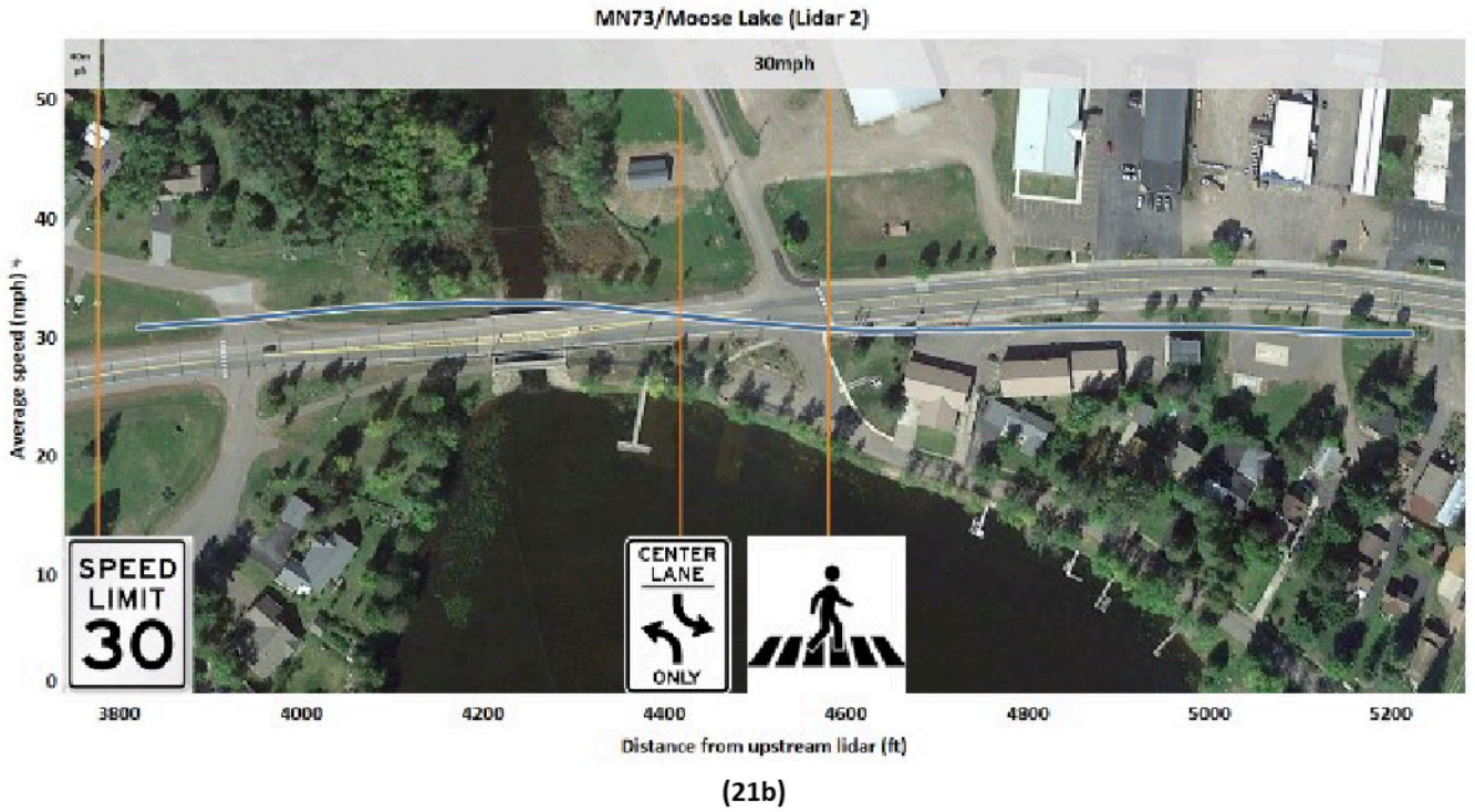
Figure 21 Average Speed Profile as Vehicles Transit from 55-40-30 mph on MN73/Moose Lake Corridor
