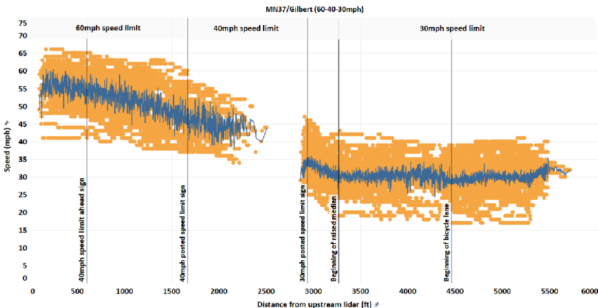
Figure 4 Speed Profile Showing Speed Reduction as Vehicles Approach MN37/Gilbert.
