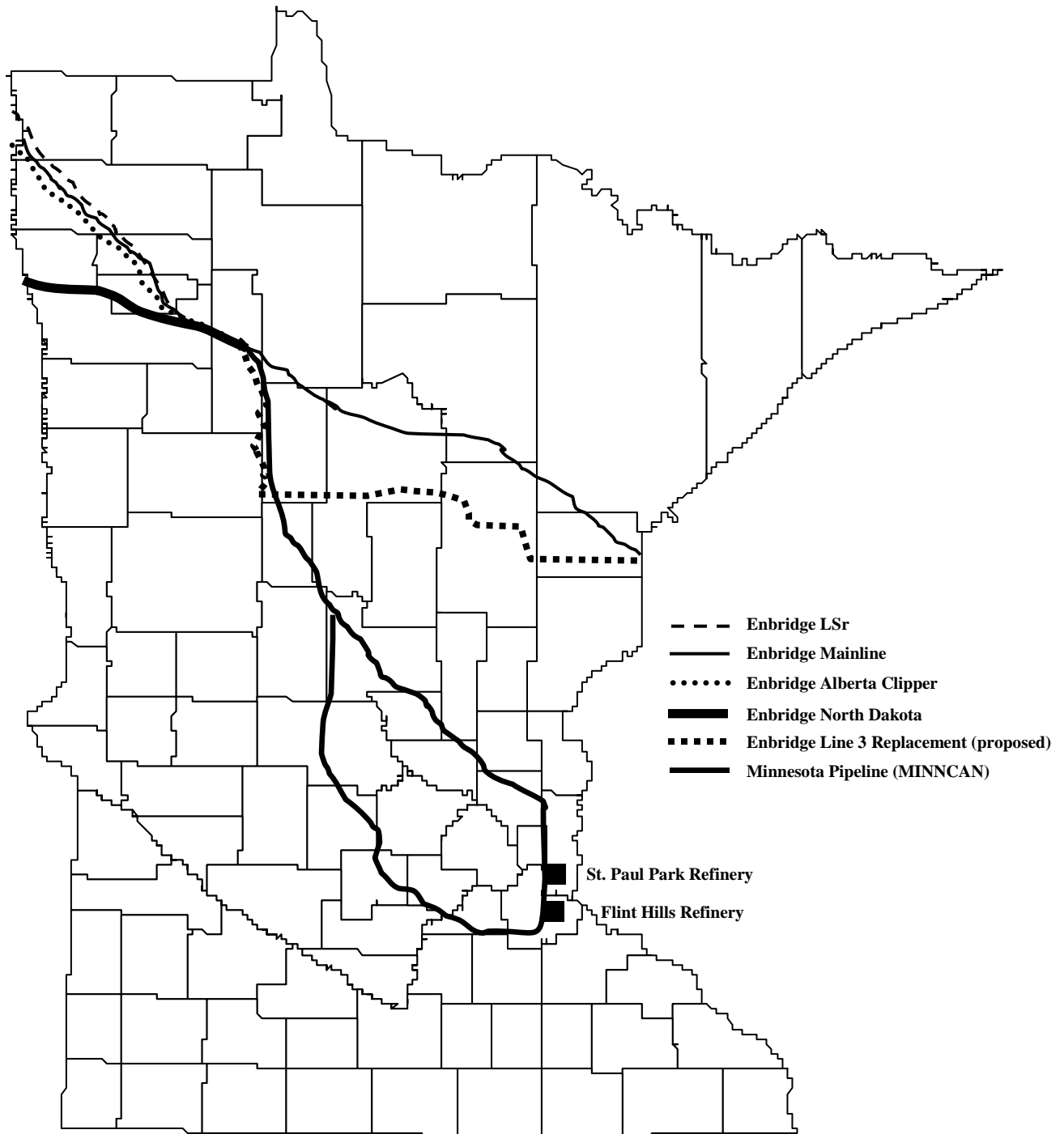
Figure 2: Crude Oil Pipelines and Petroleum Refineries
