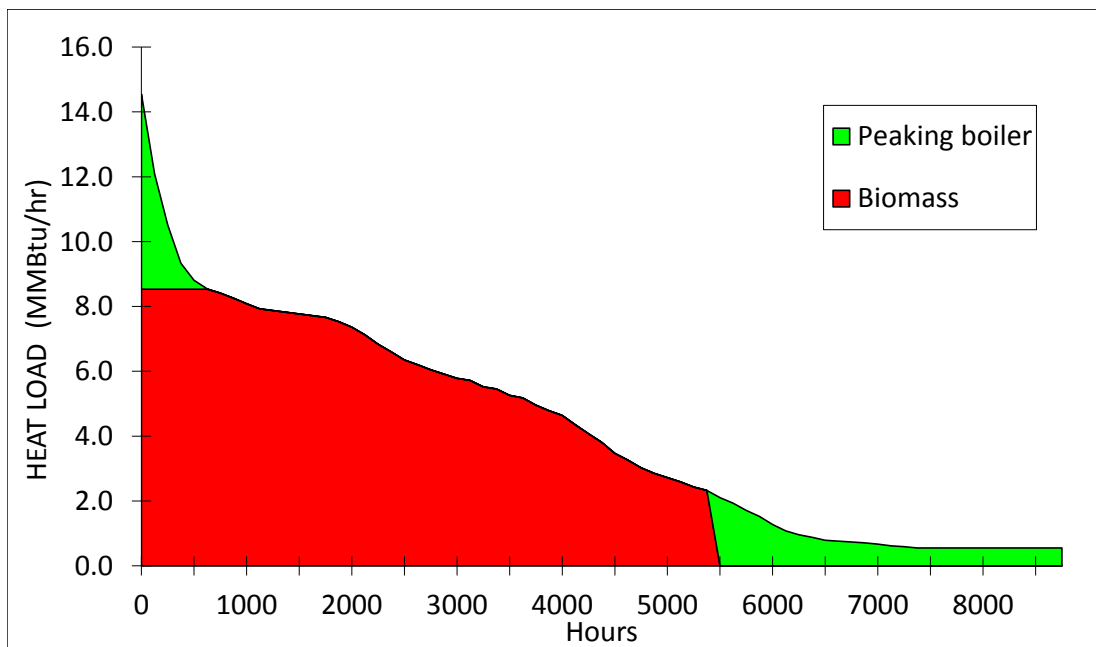
Figure 6. L6 Scenario Heat Production Duration Curve
