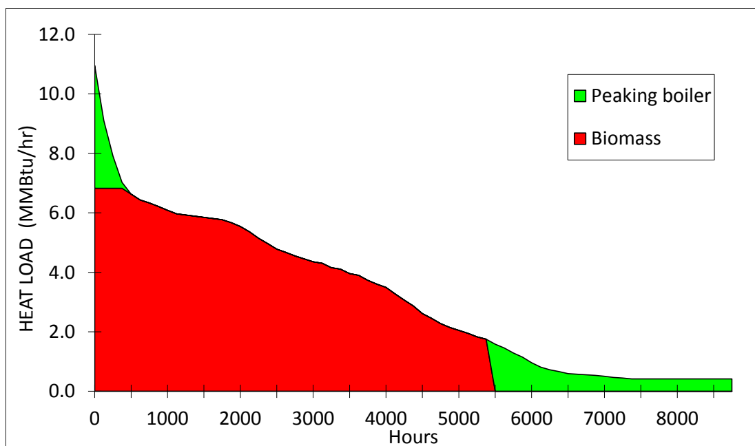
Figure 7. Hybrid Scenario Heat Production Duration Curve
