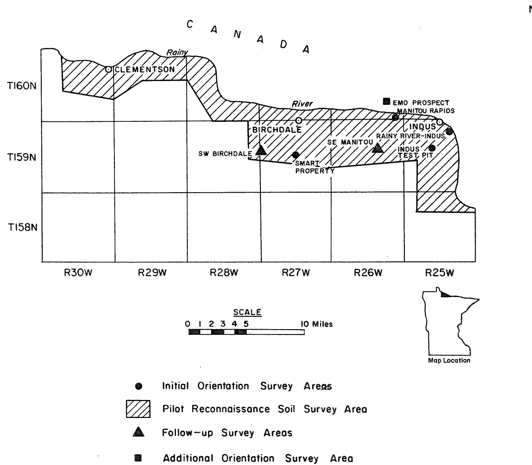
FIGURE 1: Map showing location of geochemical surveys in northwestern Koochiching and northeastern Lake of the Woods Counties, Minnesota
