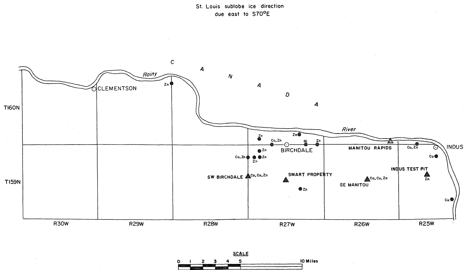
FIGURE 4: High metal values in Ah, B or C-horizon samples - Pilot Reconnaissance Soil Survey
