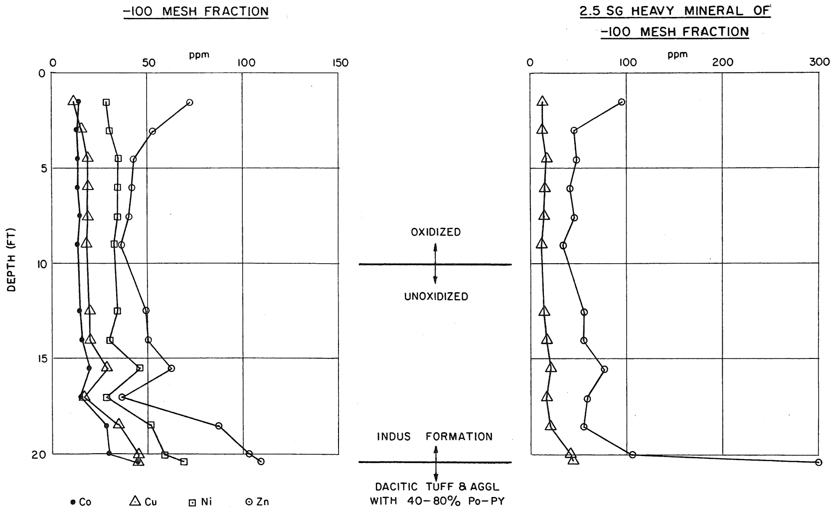
FIGURE 3: Trace metal profiles of drill hole IH-10 from Indus Test Pit
