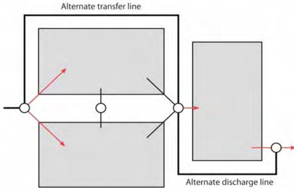
Figure 2: Two-cell non-aerated stabilization pond
