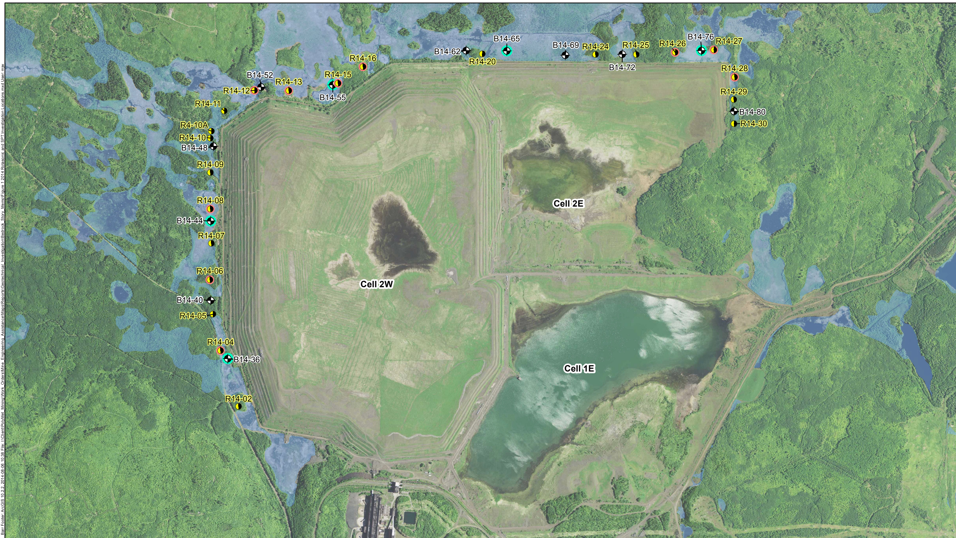
Figure 1 2014 ROTASONIC AND SPT INVESTIGATION LOCATIONS NorthMet Project PolyMet Mining Inc. Hoyt Lakes, Minnesota
