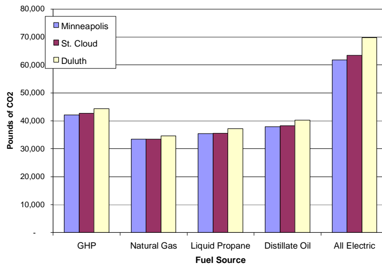
Figure 161: Annual CO2 Emissions for Small Residential New Construction Building with Respect to Heating Fuel
